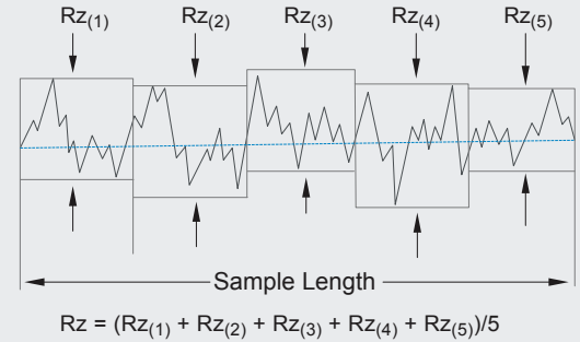
Rz – Surface Finish Measurement
