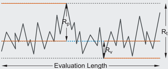
Rt – Surface Finish Measurement
